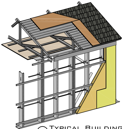
TYPICAL BUILDING ASSEMBLY
